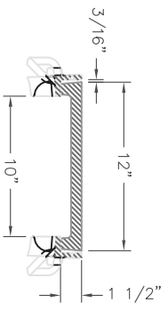
R-4999-CX TYPE "E" LID WITH TYPE "B" FRAME TYPICAL SECTION
